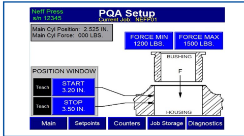
Force/Distance Monitoring
