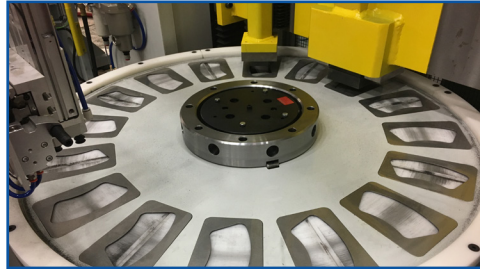
Indexers
